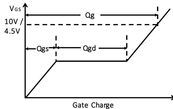
Figure 8. Gate Charge Waveform
