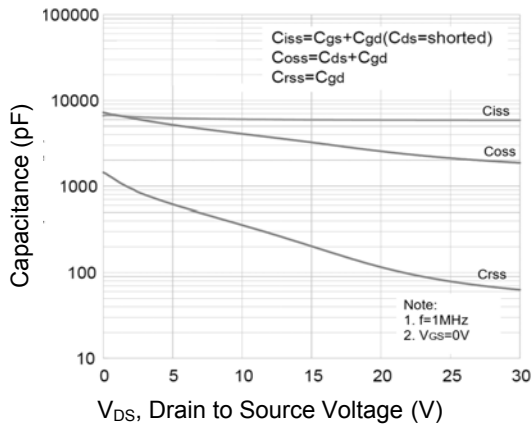
Figure 7. Capacitance Characteristics
