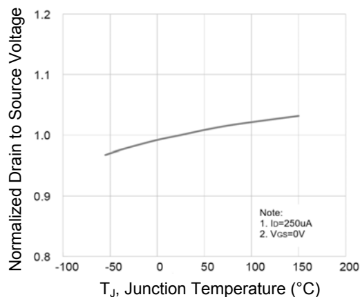
Figure 5. Normalized BV_{DS} vs. T_J
