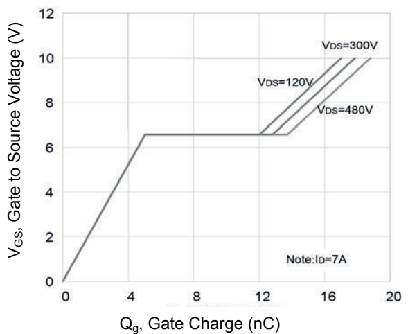
Figure 6. Gate Charge
