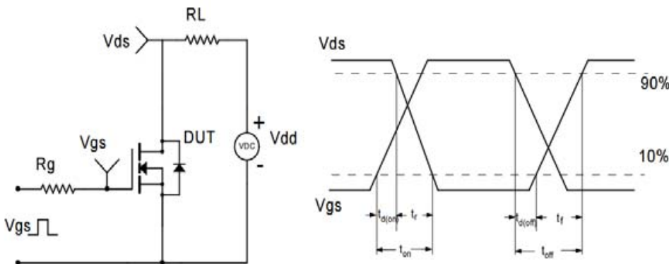
Figure 10. Switching Time Test Circuit and Waveforms
