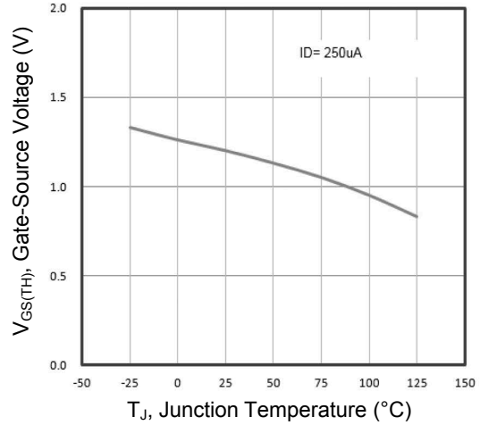
Figure 2. Normalized V_{th} vs. T_J
