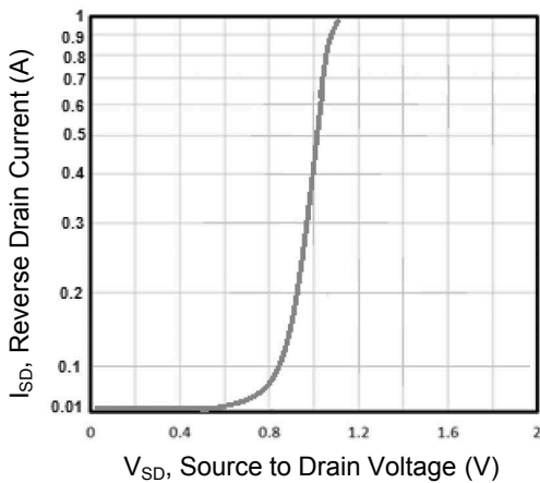
Figure 5. Typical Source to Drain Diode Forward Voltage
