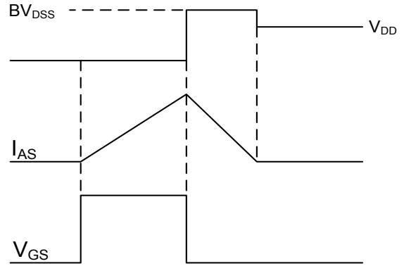
Figure 8. EAS Waveform
