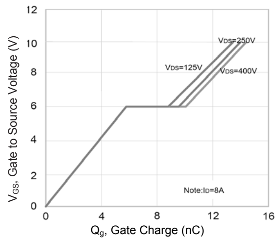
Figure 6. Gate Charge
