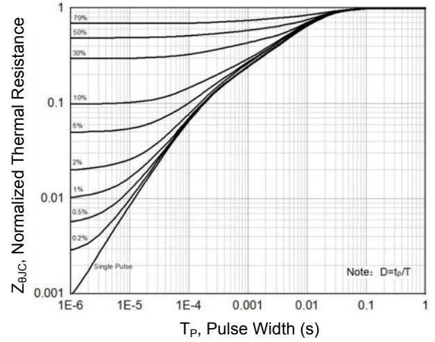
Figure 14. Transient Thermal Impedance vs. T p
