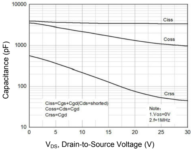
Figure 7. Capacitance Characteristics
