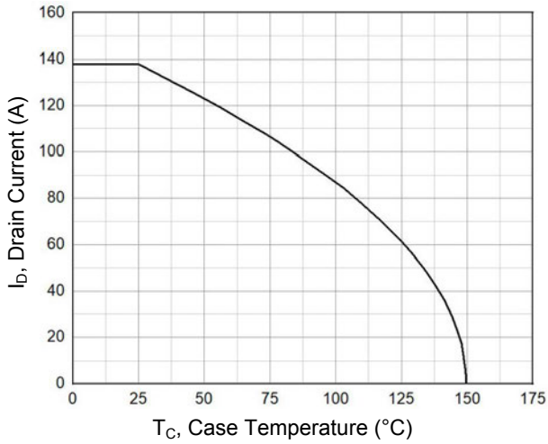
Figure 13. Drain Current vs. T c
