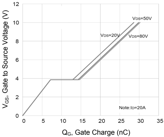
Figure 3. Gate Charge
