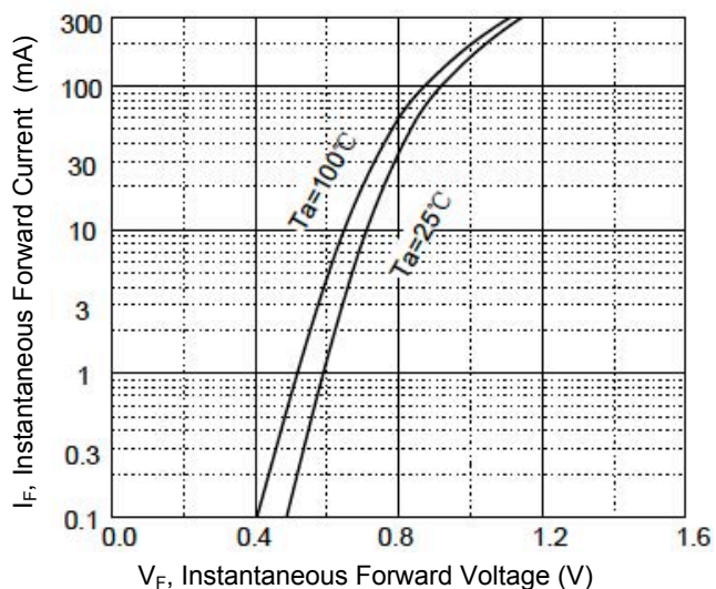
Figure 1. Forward Characteristics
