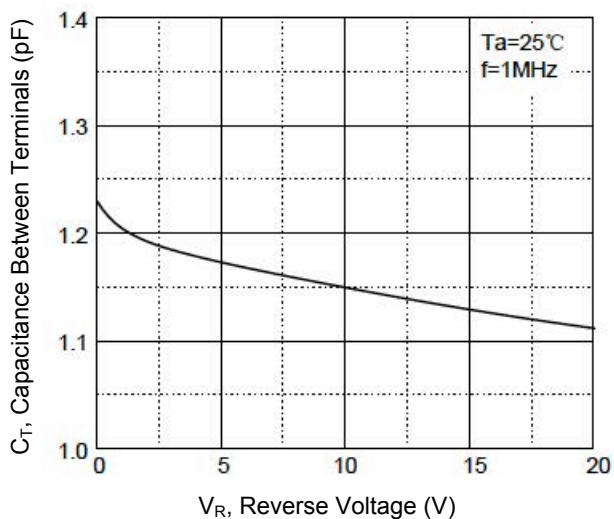
Figure 3. Capacitance Characteristics
