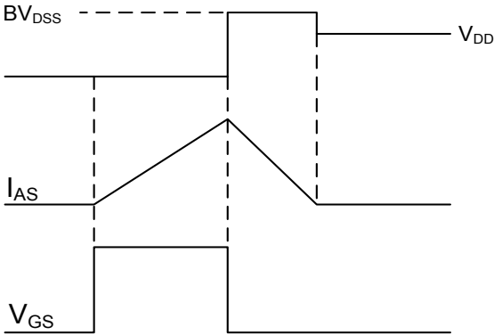
Figure 8. EAS Waveform
