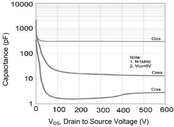
Figure 7. Capacitance Characteristics
