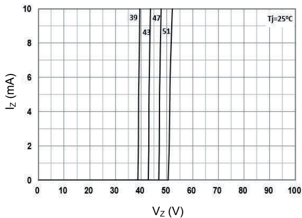
Figure 3. Breakdown Characteristics at T_j=\text{Constant} (Pulsed)
