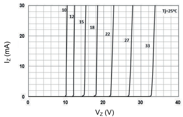
Figure 2. Breakdown Characteristics at T_j=\text{Constant} (Pulsed)
