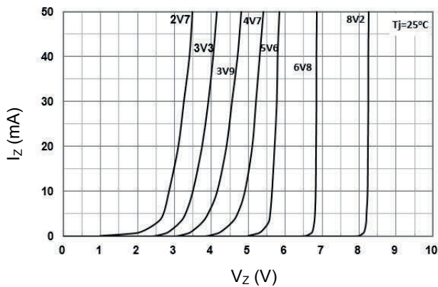
Figure 1. Breakdown Characteristics at T_j=\text{Constant} (Pulsed)
