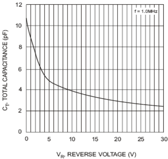
Figure 3. Capacitance Characteristics
