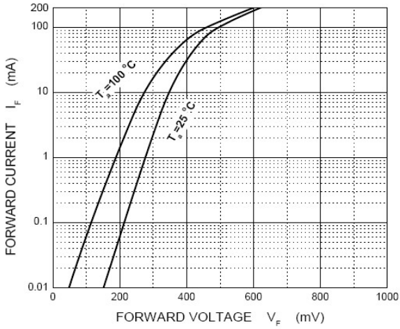
Figure 1. Forward Characteristics
