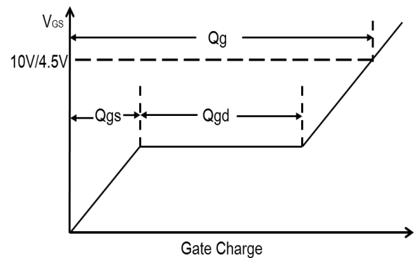
Figure 12. Gate Charge Waveform
