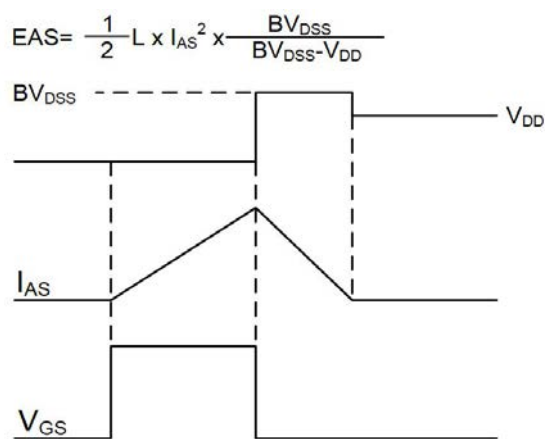
Figure 12. EAS Waveform
