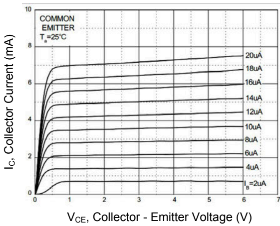
Figure 1. Static Characteristic
