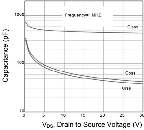
Figure 7. Capacitance Characteristics
